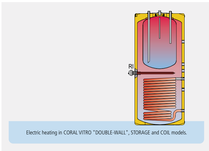
"RI" HEATING ELEMENTS: Threaded immersion heating elements for primary heating circuit, in CORAL VITRO "DOUBLE-WALL" models.
