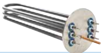
"RB" HEATING ELEMENTS: Flanged heating element for CORAL VITRO "SINGLE-WALL", STORAGE AND COIL models.
